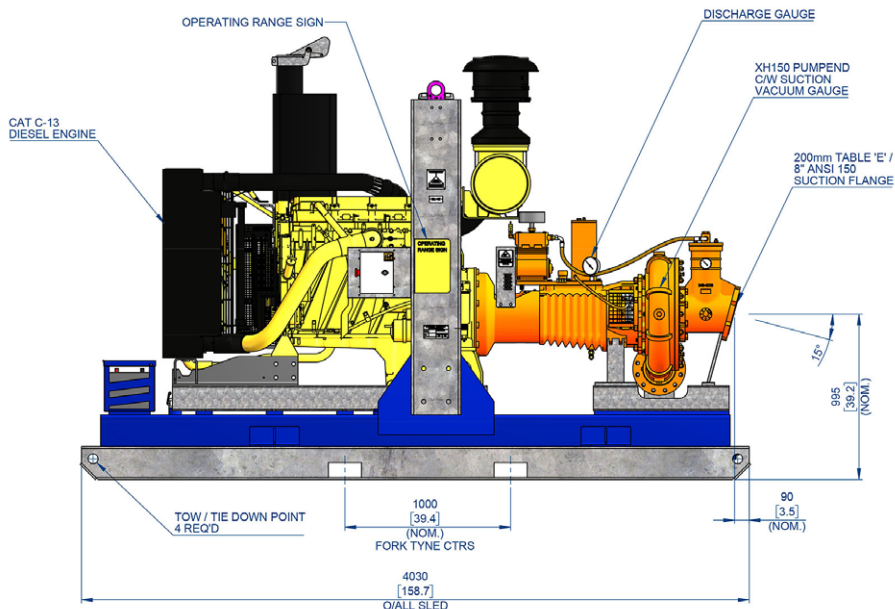
ELEVATION VIEW
